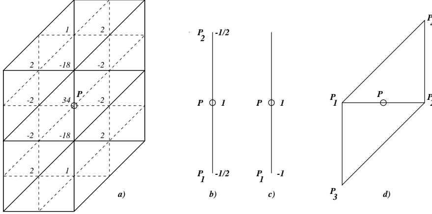
Figure 1.1 Masks for \psi_v : a) L_2 -semiorthogonal prewavelet system, b) 3-point HB-system, c) 2-point HB-system, and d) notation for Example 5.
