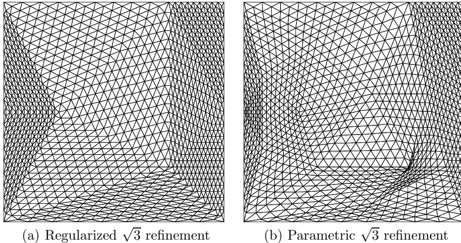
Figure 8: We compare our regularized \sqrt{3} refinement with parametric) \sqrt{3} refinement. We applied 5 steps of refinement to the irregular initial triangulation \Delta_0 from Figure 7 (b). Parametric \sqrt{3} refinement, where always the barycenters of the triangles are inserted, degenerates in this case.
